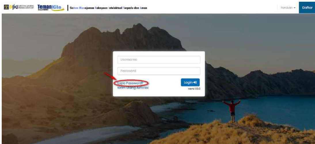
Gambar 7 Lupa Password
